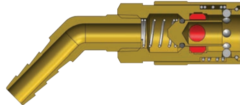
CM-Series Industrial Mold Interchange Valved Coupler (45° Hose Barb)
