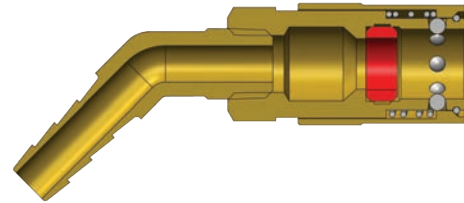
CM-Series Industrial Mold Interchange Unvalved Coupler (45° Hose Barb)
