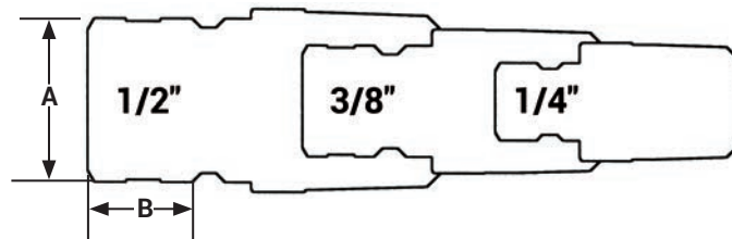
CM-Series Profiles
