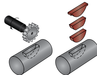
Woodruff Key
