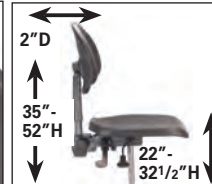
BACK/SEAT HEIGHT AND ANGLE ADJUSTMENTS
