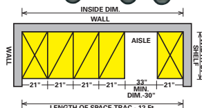
TOP VIEW SC795978
