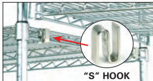
Two "S" hooks are used to connect add-on wire shelf to starter wire shelf.
