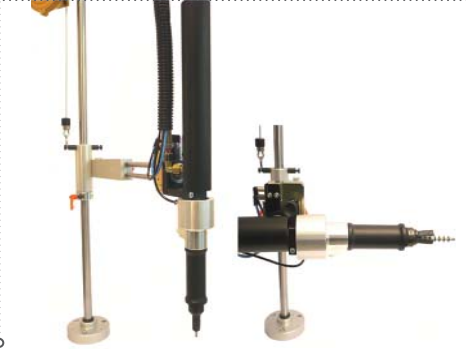
RK-753-P3 PANTOGRAPH RIVETING TOOL
