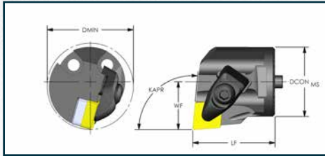
PULLBACK Clamp Negative 80° Diamond (KAPR 95° Lead)
