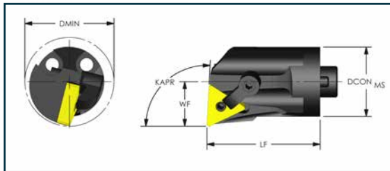
Negative Triangle ( KAPR: 93°)
