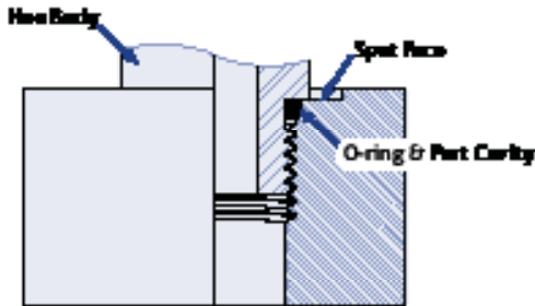
Straight SAE ORB
