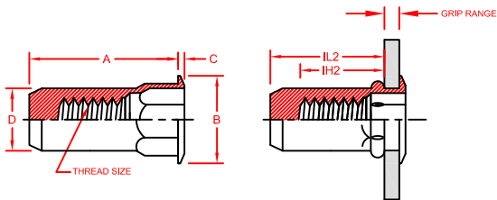
IHF-CE SERIES CLOSED END
