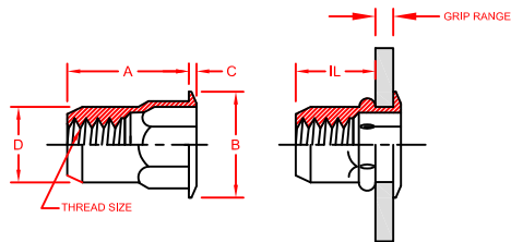
IHF SERIES OPEN END
