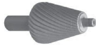
REF. # 50916 Here is the cutter used in the router to the left. A bearing is put on the end of this cutter to use as a guide. The tool bevels the inside of PVC tubing.
