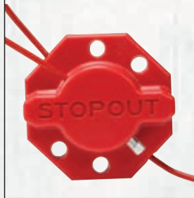
Cinch closed position with holes aligned.
