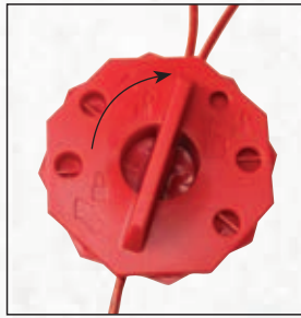
Turn the hasp halves to cinch cable.
