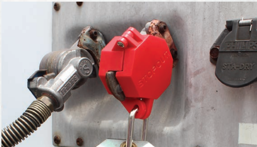
Close device over Glad Valve and secure with padlock (shackle diameter up to 9/32") and tag.
