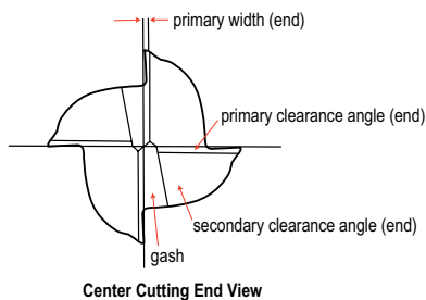
Center Cutting End View
