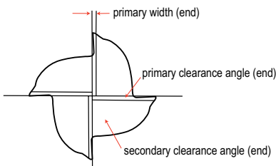
Non-Center Cutting End View
