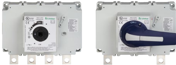
2 Pole (Type 2E) Dc Ungrounded
