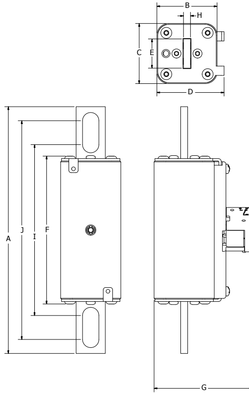
Figure 2. Bolted-blade style
