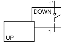
Type 4D (1 Pole)
