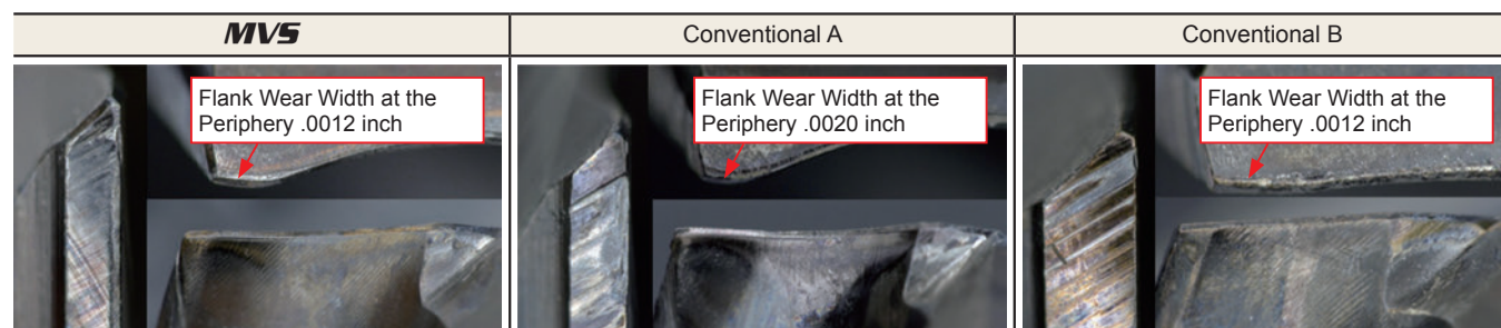
Damage of the Cutting Edge after 180 feet of Machining
