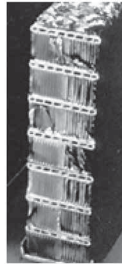
More passages closer together. CANNOT be flushed completely!
