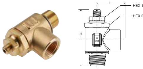
FC703 Threaded Port Meter Out Metal Flow Control – NPT
