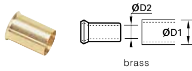
brass
