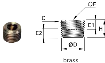
brass
