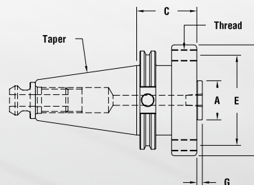
Boring Ring Holder PC7-17BR2 shown here.
