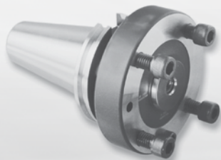
Boring Ring Holder PC7-17BR2 shown here.
