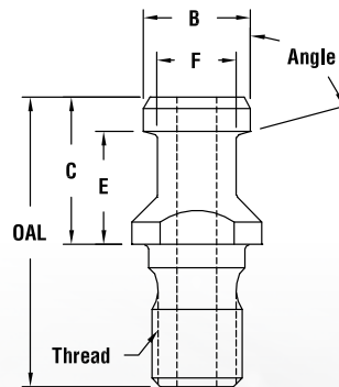
DIN50ATRK shown here.
